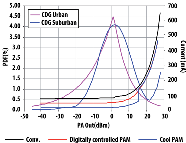
Figure 13. CDMA Power Distribution Function
