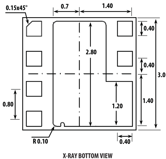
Figure 8. Package Dimensional Drawing and Pin Descriptions (All dimensions are in millimeters)
