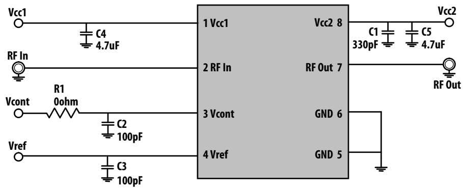
Figure 6. Evaluation Board Schematic
