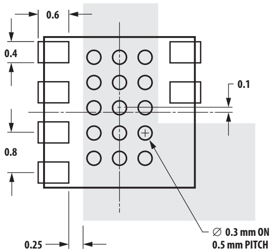
Figure 14. Metallization
